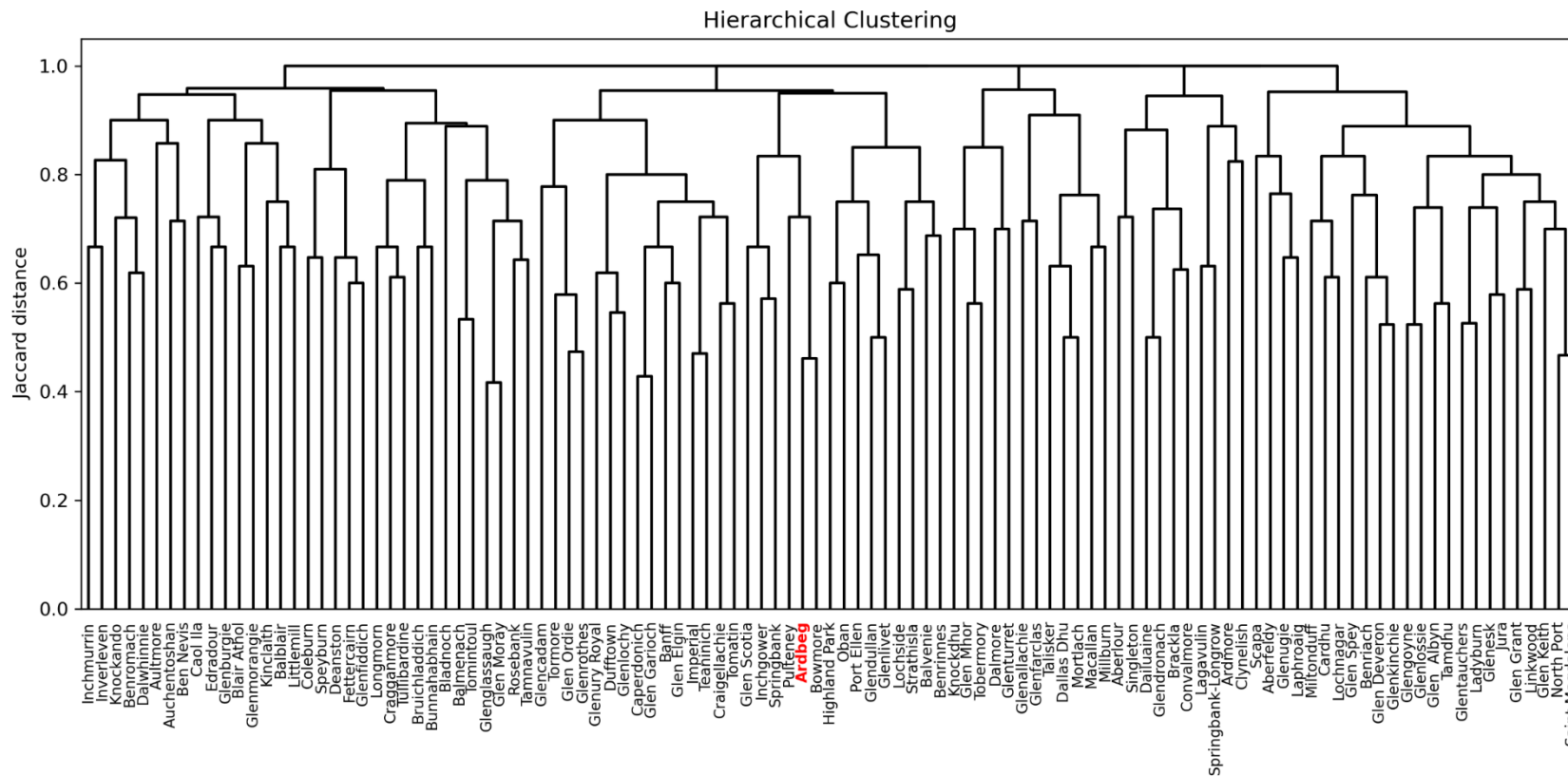
Dendrogram for whisky example
